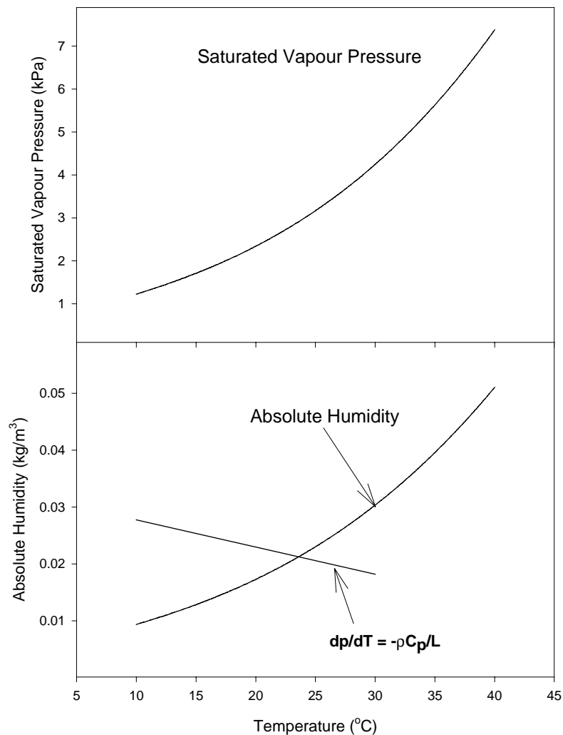
Figure 3.4.1 Variation of saturated vapour pressure (upper graph) and absolute humidity (lower graph) with temperature at atmospheric pressure P=100kPa
