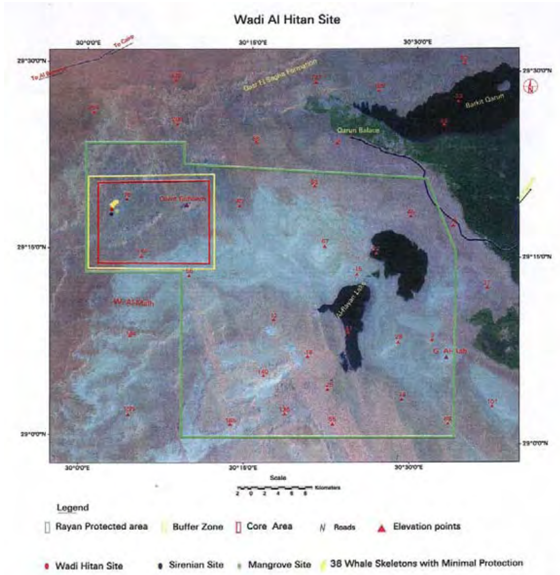
Fig. 1 – Map produced of satellite image of Wadi Al-Hitan (Whale Valley), Wadi El-Rayyan Protected Area, Faiyum Governorate, proposed World Heritage Site showing approved boundaries of core area (red rectangle) and buffer zone (yellow rectangle). The boundaries of the Wadi Al-Rayyan Protected Area (WRPA) are shown by a green line. Scale of A4 reduction: ~ 1:579,000. Map prepared by EGSM (Egyptian Geological Survey and Minerals Authority).
